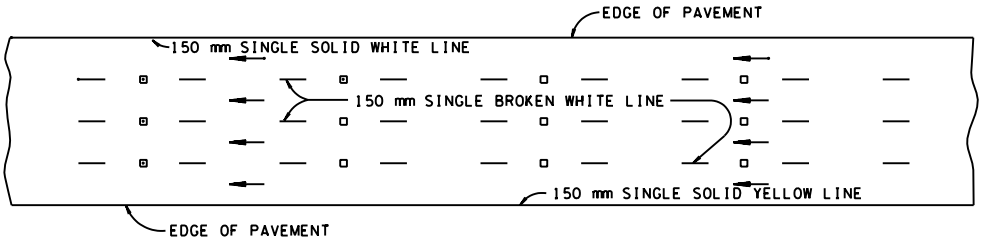
TYPICAL FOUR LANE
