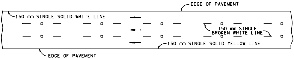
TYPICAL THREE LANE
