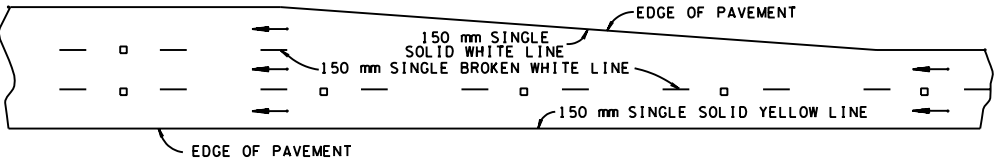
TYPICAL SHOWING BEGINNING OF ADDITIONAL LANE
