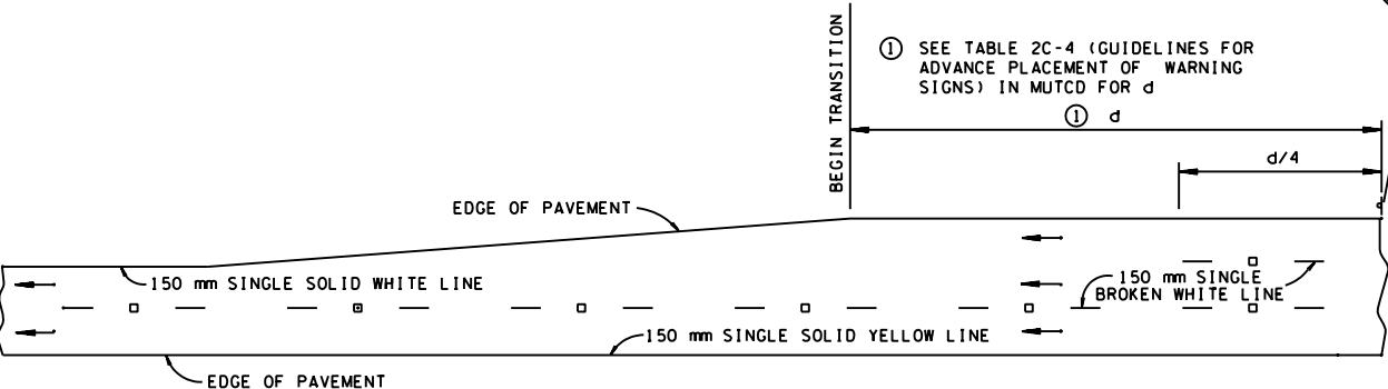
TYPICAL SHOWING ENDING OF ADDITIONAL LANE
